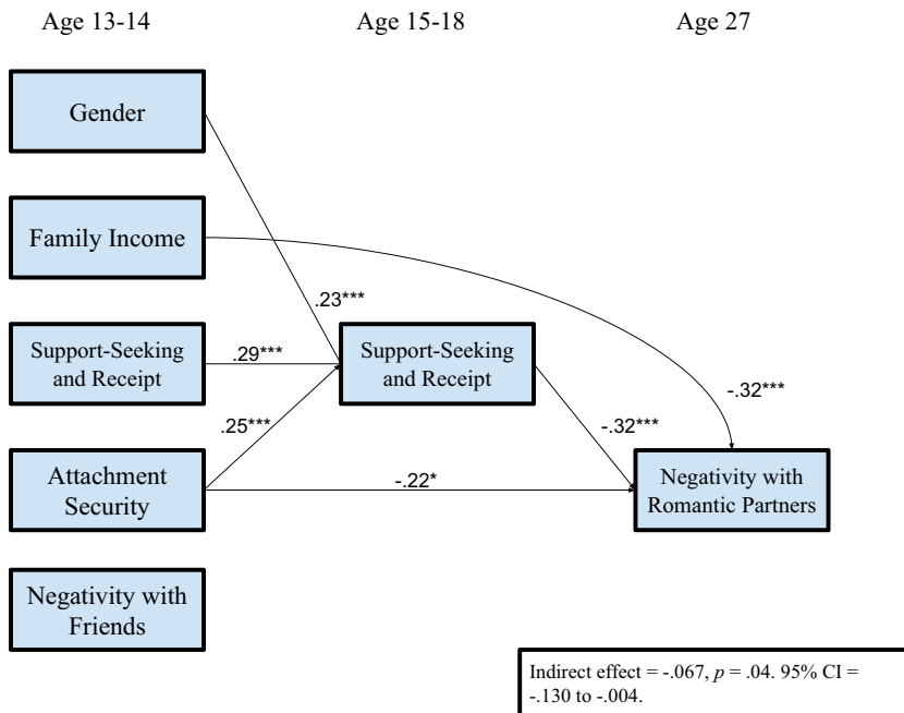
Figure 1. Mediation model of attachment security at 14 to negativity with romantic partners at age 27, via difficulties seeking and receiving support with close friends from ages 15–18.
